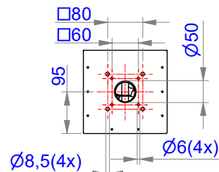
Bottom plate for MCVi-1
