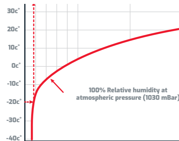
MOLLIER DIAGRAM
